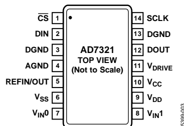
Figure 3. Pin Configuration
